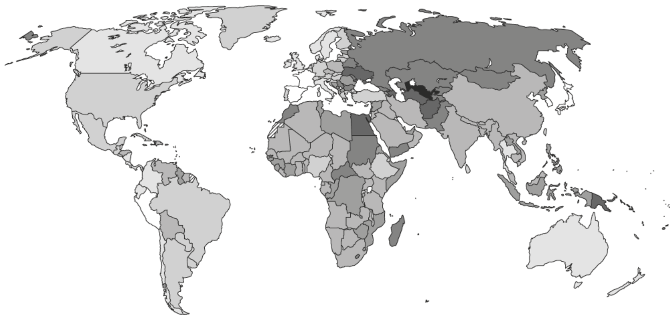
Fig. 2 – Global distribution of cardio-vascular disease (CVD) mortality, 2017
