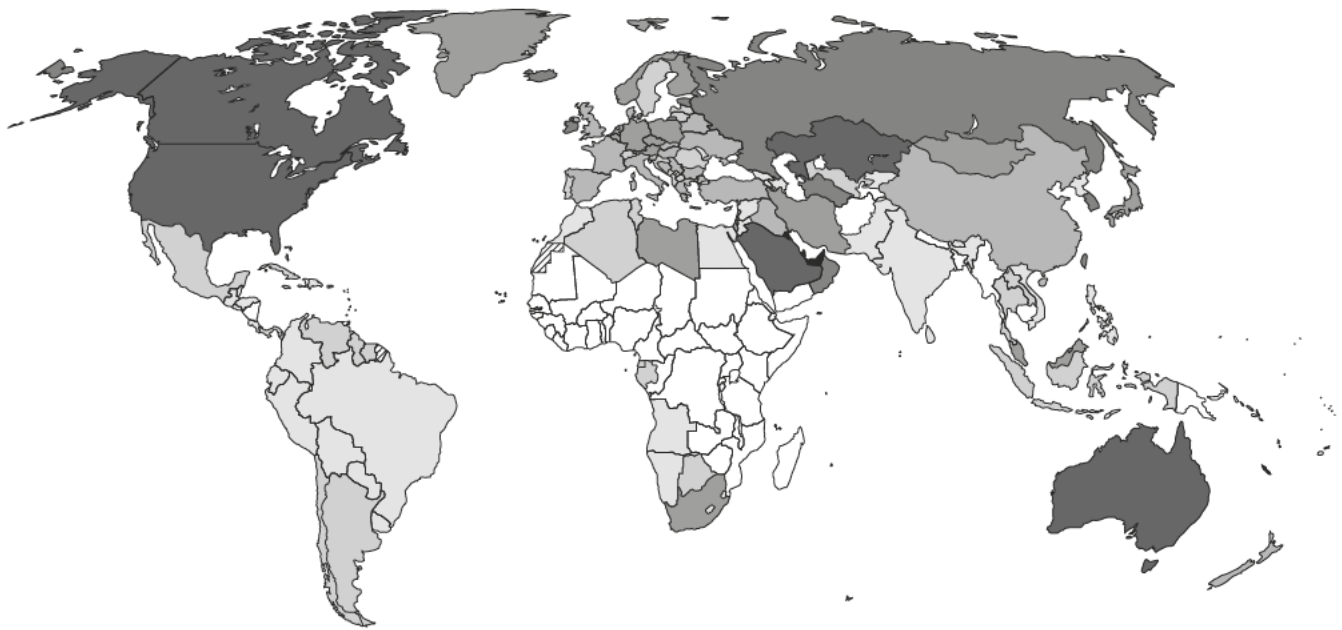
Fig. 1 – Global distribution of carbon dioxide emissions per capita, 2018
