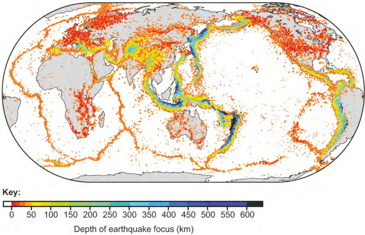
Fig. 5 – Global distribution of earthquakes from 1960 to present
