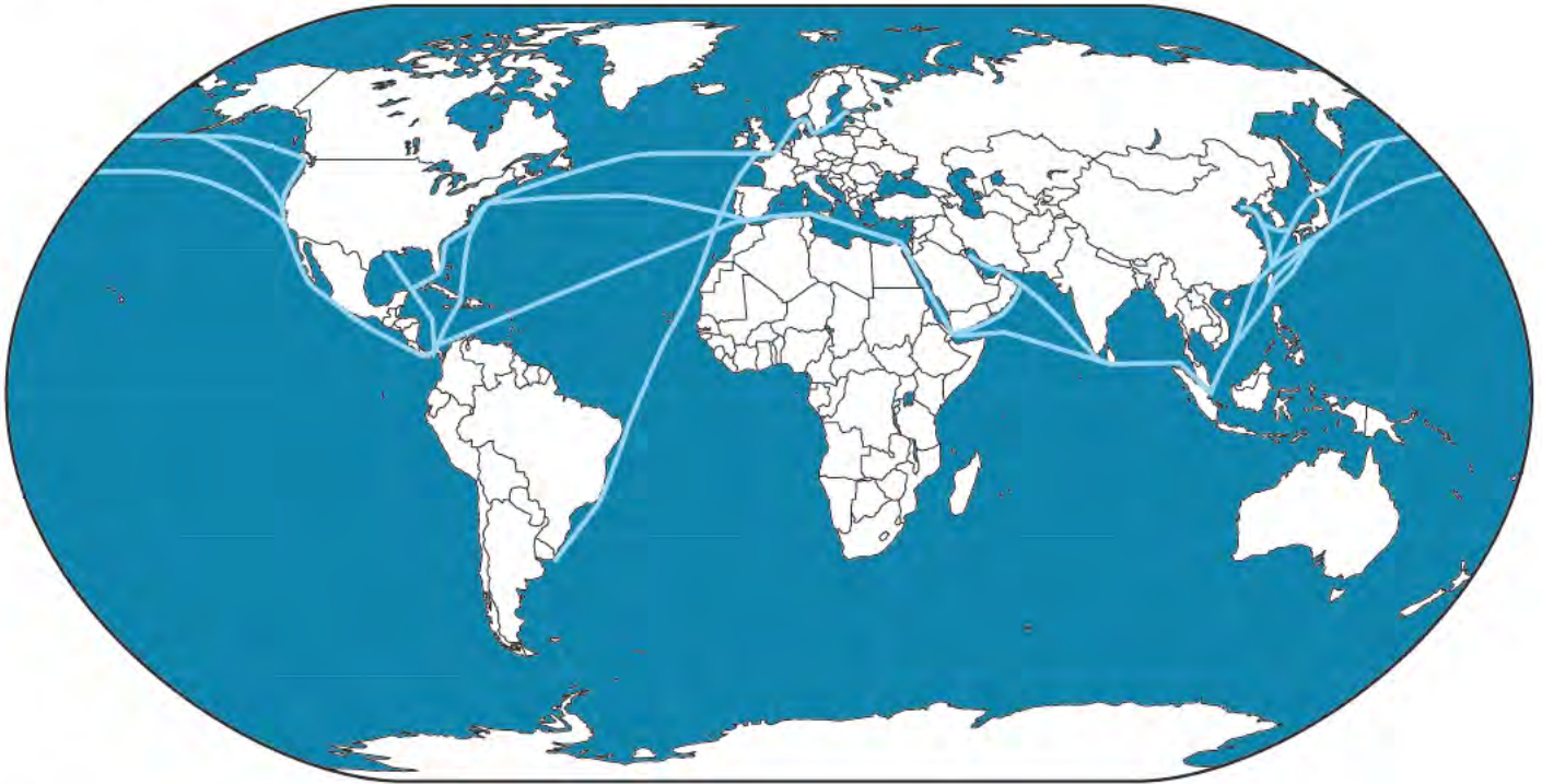
Fig. 3 – Global pattern of principal shipping routes across the oceans
