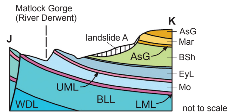
CROSS-SECTION SHOWING THE GENERAL RELATIONS OF THE ROCKS ALONG THE LINE (J-K) DRAWN ON THE GEOLOGICAL MAP
